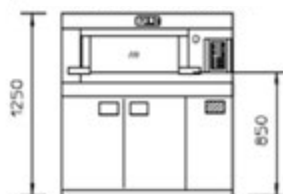
Forno a 1 camera - 1 deck oven
