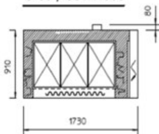
Forni standard - Standard ovens
