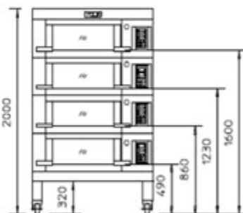
Forno a 4 camere - 4 decks oven
