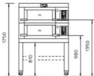
Forno a 2 camere - 2 decks oven
