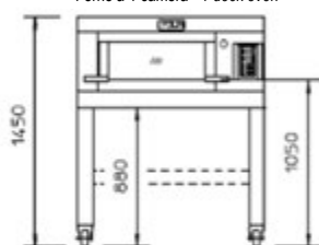
Forno a 1 camera - 1 deck oven
