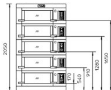
Forno a 5 camere - 5 decks oven
