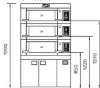
Forno a 3 camere - 3 decks oven
